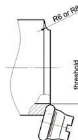
R6 & R8 J-groove available with optional milling heads
